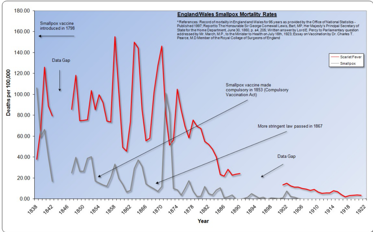
G 5.3: England and Wales smallpox and scarlet fever death rates from 1838 to 1922.
